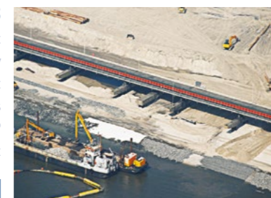
2008 JadeWeserPort Germany Revetment HaTe® Nonwovens Tektoseal® Sand mat
